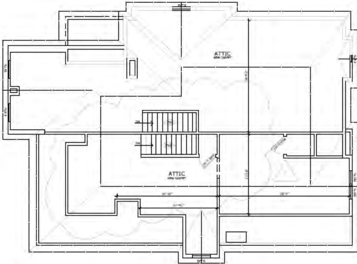
01 THIRD FLOOR NEW PLAN
