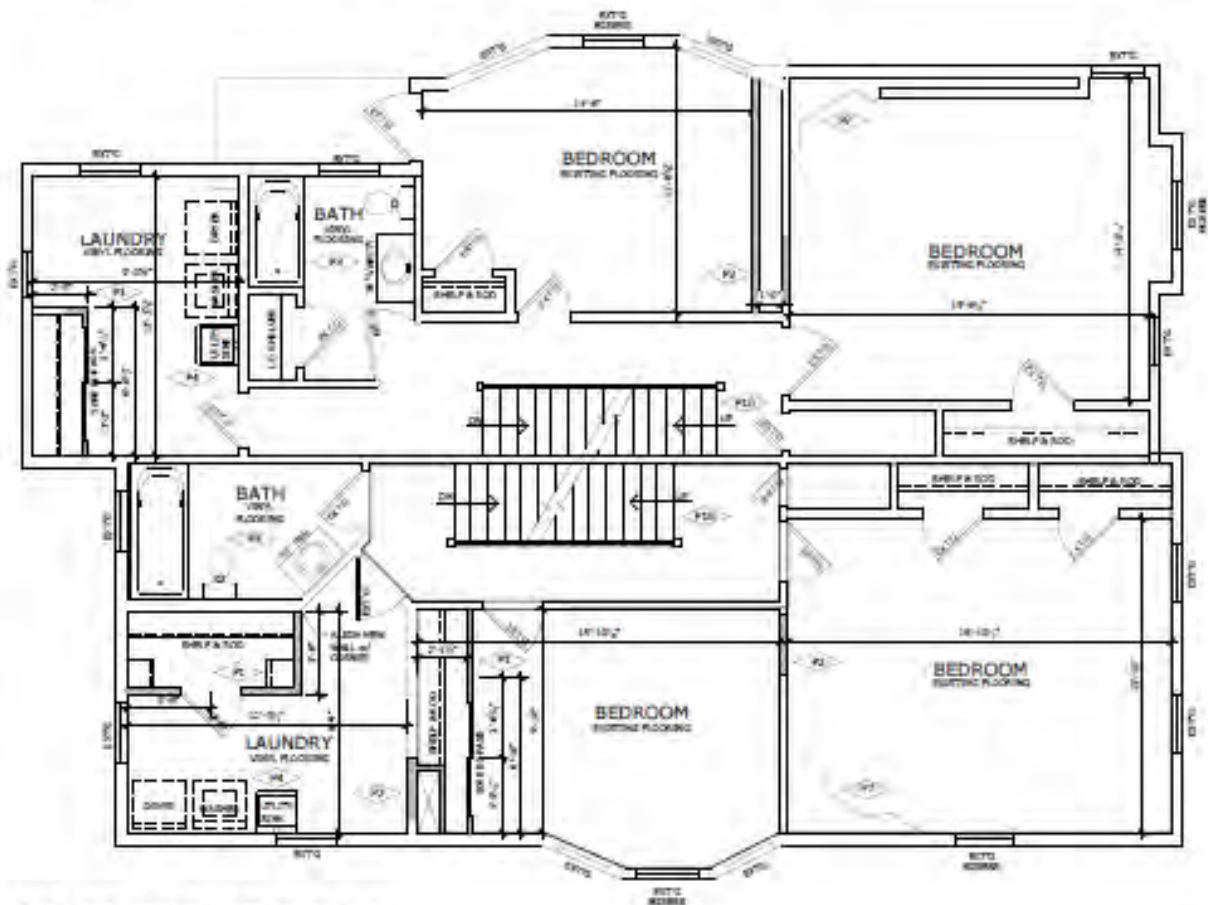
01 SECOND FLOOR NEW PLAN
